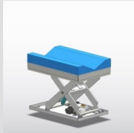
Prism support
