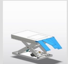
Access ramp manually operated, divided design
